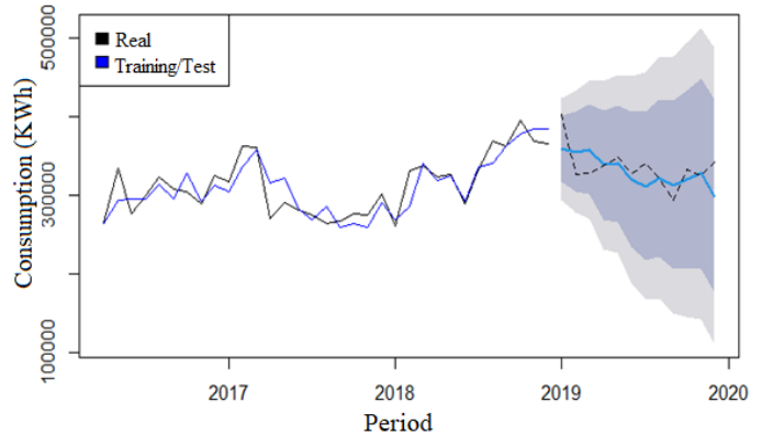
Figure 8. Graph of the forecast using the ARIMA(1, 1, 16)(0, 0, 1) model.
