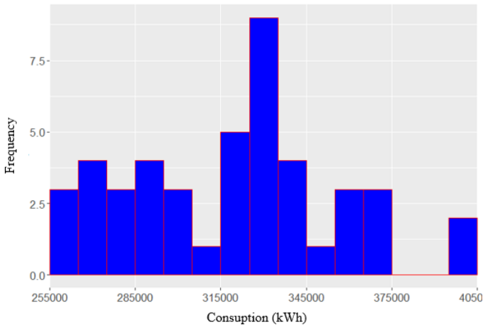
Figure 6. Graph Histogram Total Consumption kWh.
