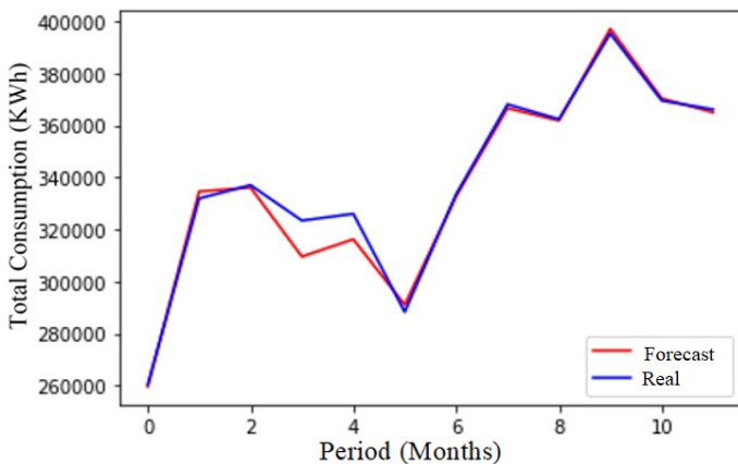
Figure 9. Validation graph (2017-2018) of the LSTM model with 10 cells in the first hidden layer and 5 cells in the second.
