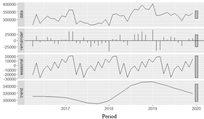
Figure 7. Decomposition of the Total Consumption series into the patterns of a time series (trend, seasonality and randomness).
