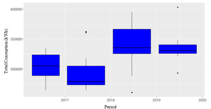
Figure 5. Box Plot of total annual consumption in kWh.
