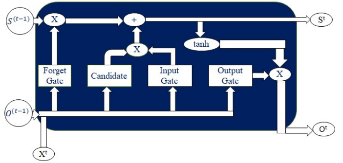
Figure 2. Representation of a memory cell of a LSTM network.
