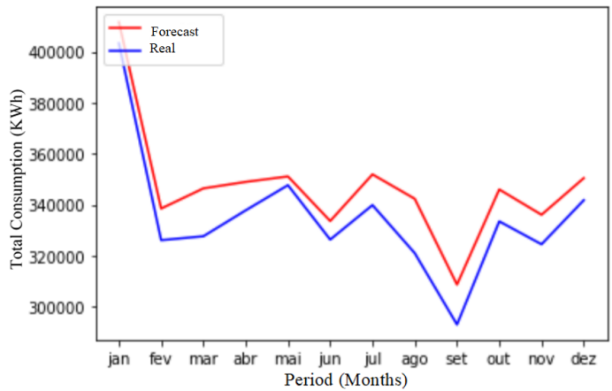
Figure 10. Test graph (2018-2019) of the LSTM model with 10 cells in the first hidden layer and 5 cells in the second.
