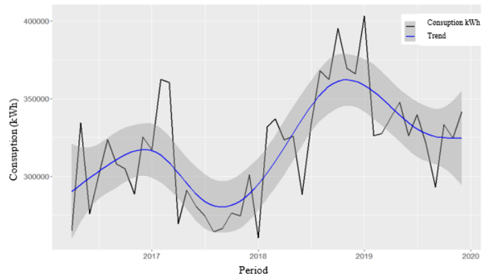
Figure 4. Total Consumption kWh series graph with trend.
